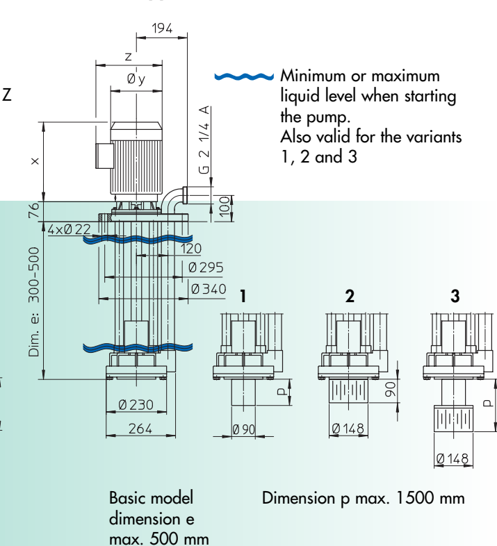
Dimensions F 716 PP2-230 and F 716 PVDF2-230
