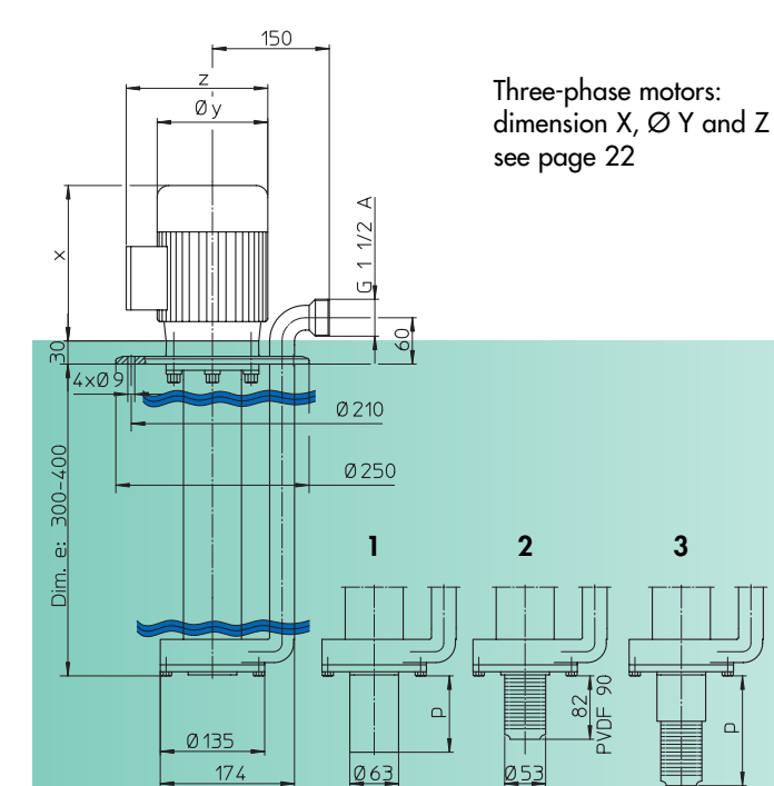
Dimensions F 716 PP1-135
