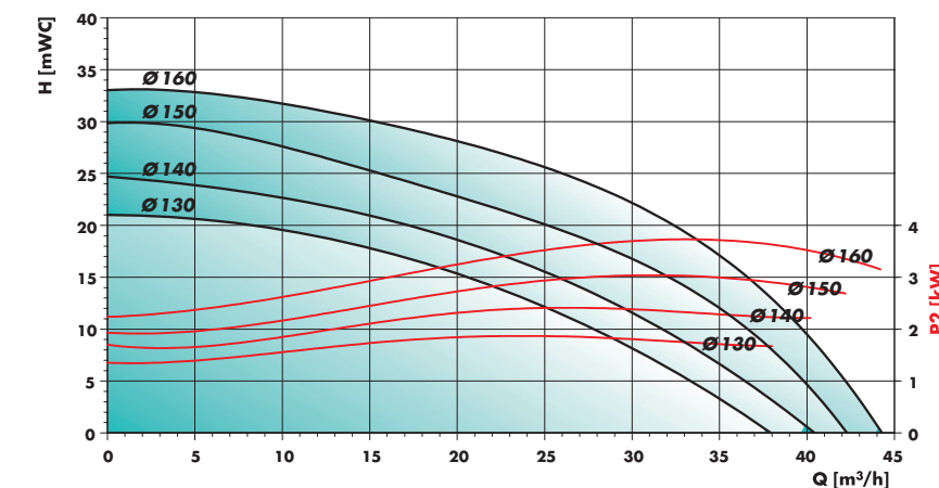
Performance chart F 706 PP-350
