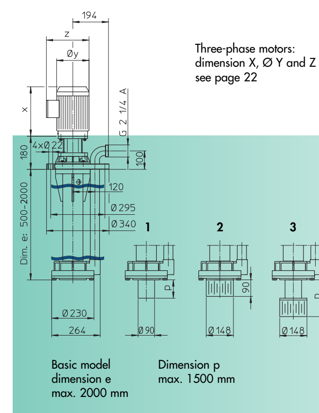
Dimensions F 706 PP-230
