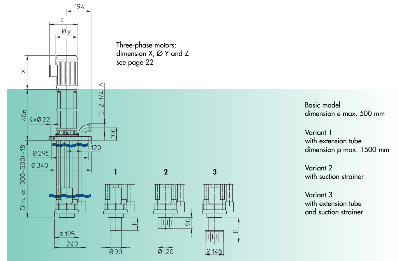
Dimensions F 726 PP2-185 and F 726 PVDF2-185
