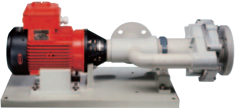
F 640 PP-230 TR mounted on base plate
