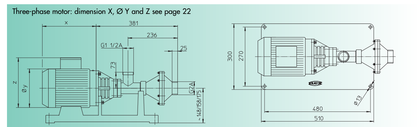
Dimensions F 640 PP-30 TR with thread connection
