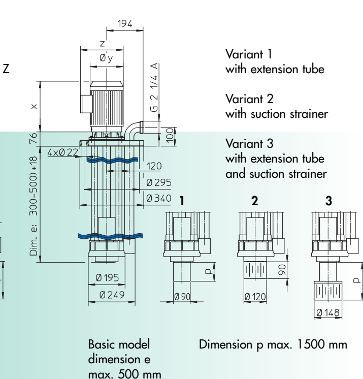
Dimensions F 716 PP2-185 and F 716 PVDF2-185
