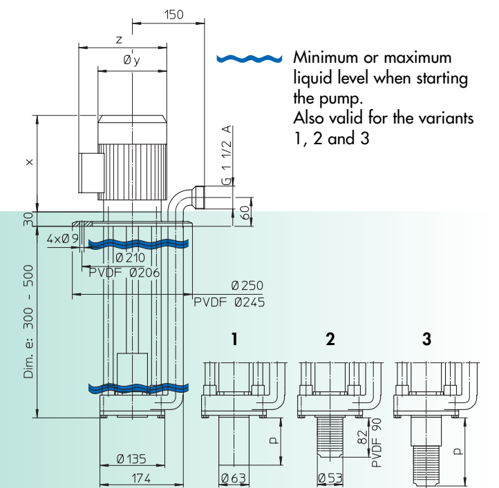
Dimensions F 716 PP2-135 and F 716 PVDF2-135
