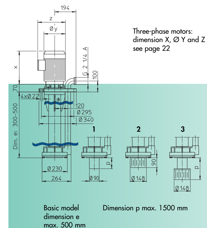
Dimensions F 716 PP1-230
