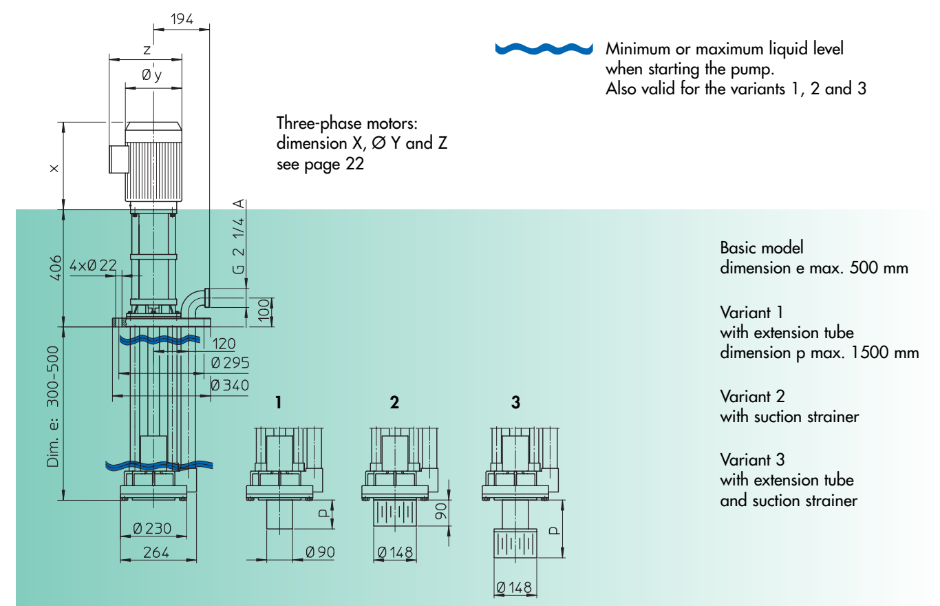
Dimensions F 726 PP2-230 and F 726 PVDF2-230
